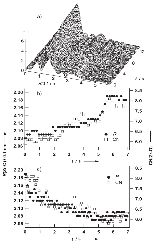
Figure 3. a) Serial k^3 -weighted energy-dispersive EXAFS Fourier transforms at the Zr K edge for \text{Pt/Ce}_2\text{Zr}_2\text{O}_8 in the oxygen-release process at 773 K. b and c) Time profiles of the coordination number (CN) and Zr–O distance ( R ) in the oxygen-storage (b) and -release processes (c) at 773 K. R \pm 0.002 \text{ nm} . \text{CN} \pm 0.7 .
