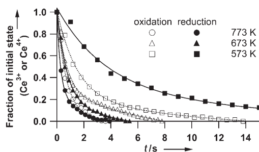
Figure 2. Time profiles of the fractions of \text{Ce}^{3+} and \text{Ce}^{4+} in \text{Pt/Ce}_2\text{Zr}_2\text{O}_x ( x=7 or 8 ) during oxygen storage and release, respectively ( \pm 0.03 ).
